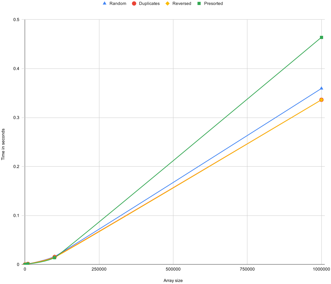
Heap Sort Time Complexity
